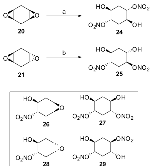
Scheme 3. Reagents and conditions: (a) \text{Bi}(\text{NO}_3)_3 \cdot 5\text{H}_2\text{O} , room temp., 20 min, 74%; (b) \text{Bi}(\text{NO}_3)_3 \cdot 5\text{H}_2\text{O} , room temp., 20 min, 71%.
