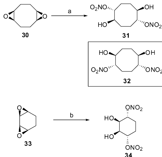
Scheme 4. Reagents and conditions: (a) \text{Bi}(\text{NO}_3)_3 \cdot 5\text{H}_2\text{O} , room temp., 16 h, 70%; (b) \text{Bi}(\text{NO}_3)_3 \cdot 5\text{H}_2\text{O} , room temp., 30 min, 85%.
